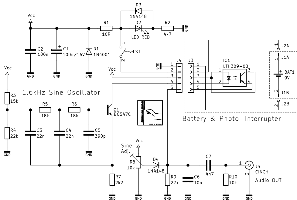
Theremin Hand to Antenna Distance Indicator Device (THADID)
